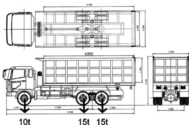
Picture 3.4. Dump Truck Vehicle Load
