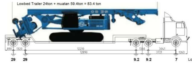
Picture 3.5. Rig Machine Soilmec load 59.4 Tons + trailer
