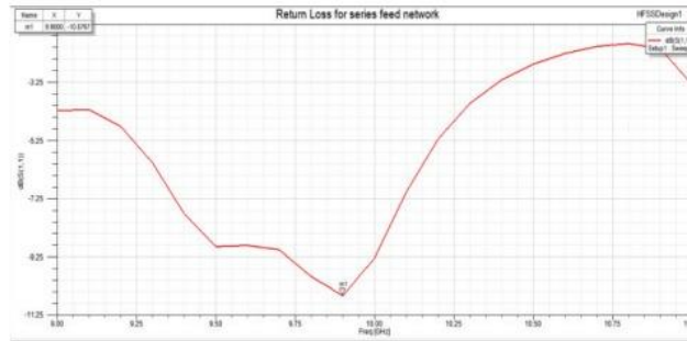
Fig. 14. Return Loss Graph For Series Feed Network
