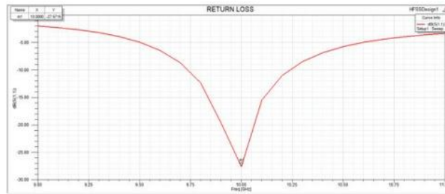
Fig. 13. Return Loss Graph For Microstrip Patch Antenna
