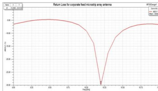
Fig. 15. Return Loss Graph For Corporate Feed Network
