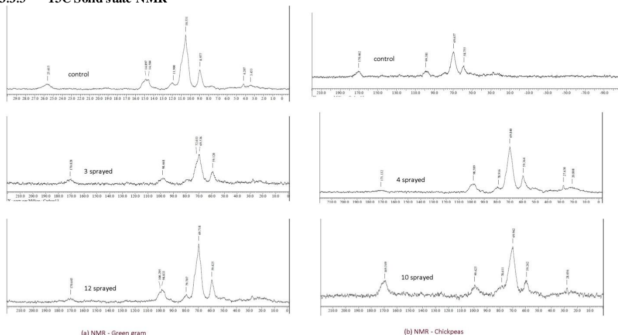
Fig 6: 13 C solid state NMR spectra
