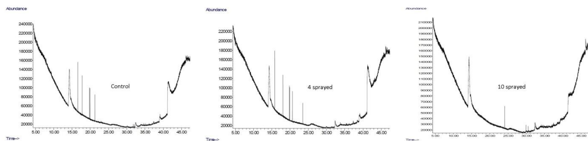
(b) GCMS - Chickpeas
