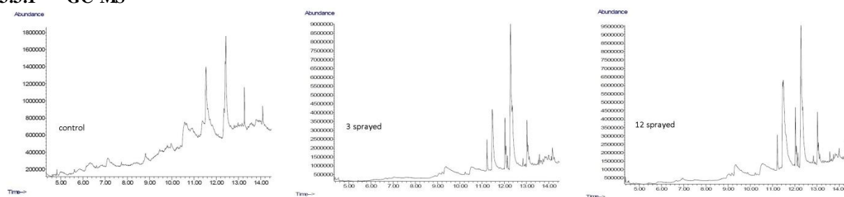
(a) GCMS - Green gram
