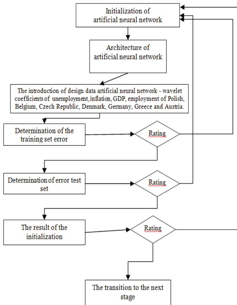
Fig. 4. Schematic of the third stage of the algorithm
