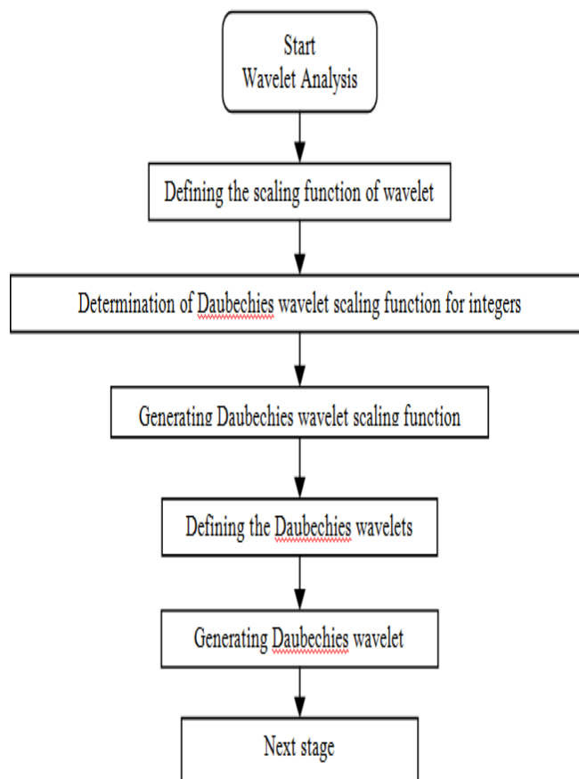
Fig. 2. Schematic of a first stage of the algorithm Source: Own.
