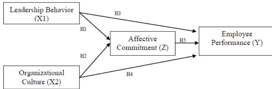
Figure 2.1. Research model
