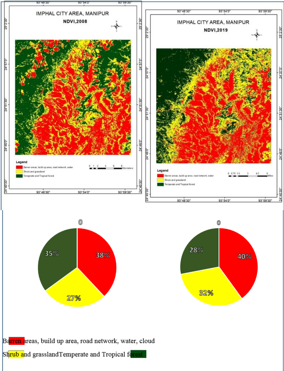
Fig. 2: NDVI threshold classification map of the 2008 and 2019
