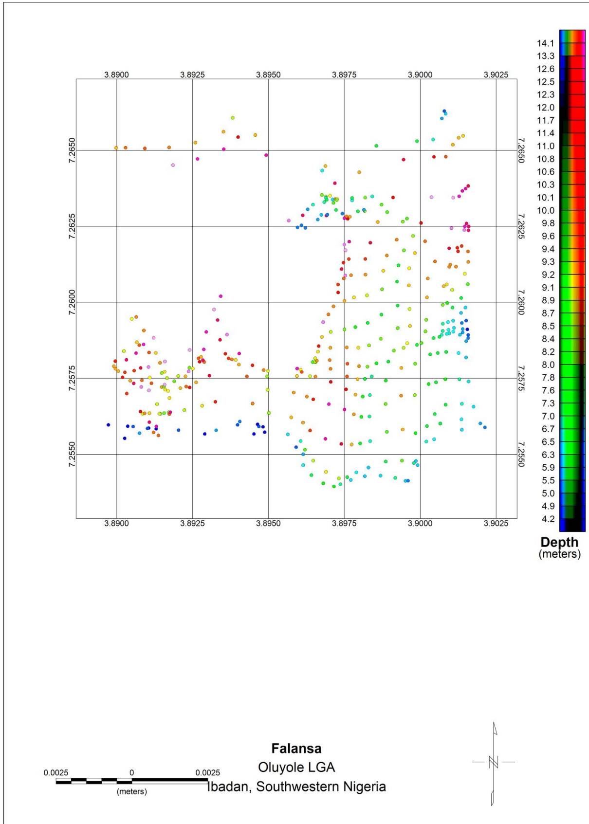
Fig. 5: Euler Solution Map for Falansa
