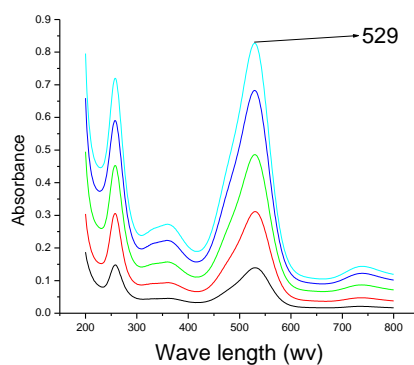
Figure ( 2 ) : The maximum absorption of ruthenium red .
