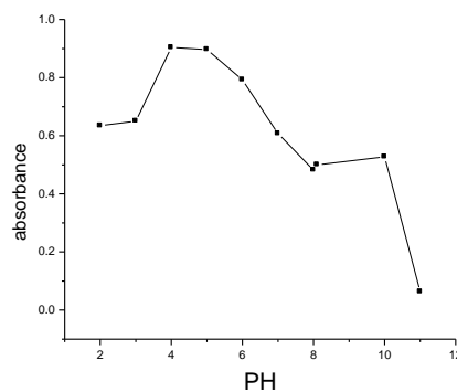
Figure ( 3 ) : The relationship between PH and Absorbance of Phenol red.
