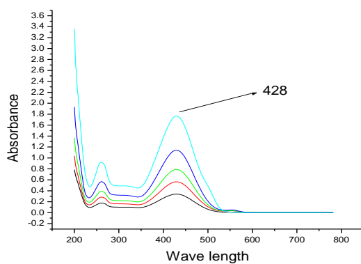
Figure ( 1 ) : The maximum absorption ( \lambda_{max} ) of phenol red .
