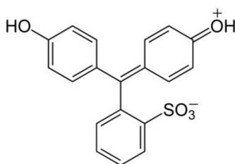
Chemical structure of phenol red .
