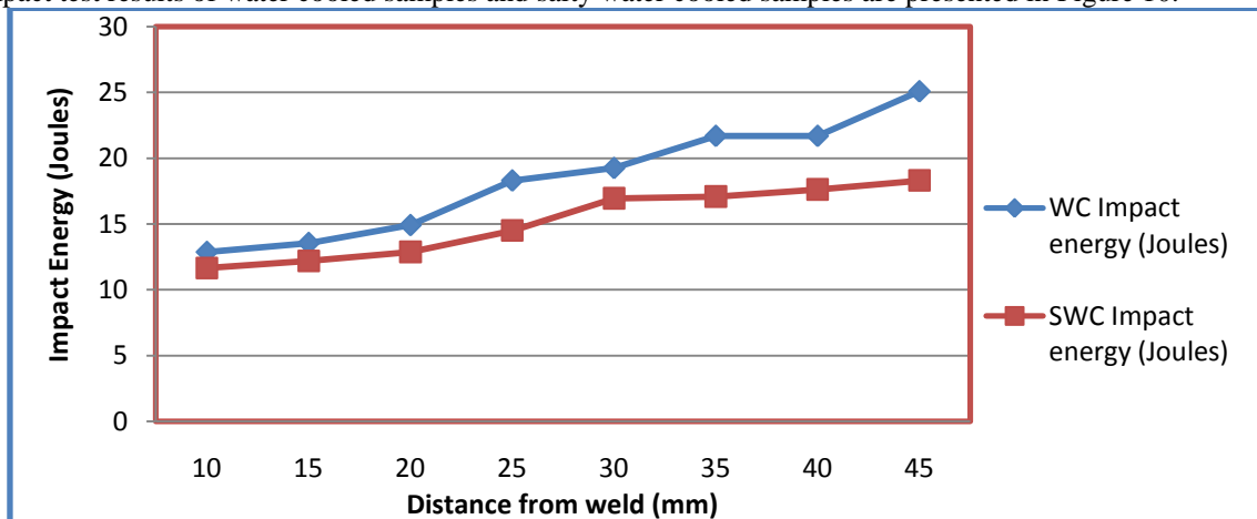
Figure 10: Variation of Impact Energy and Distance of Weld of Samples.
