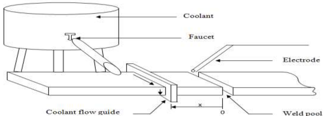
Figure 2: Experimental set-up
