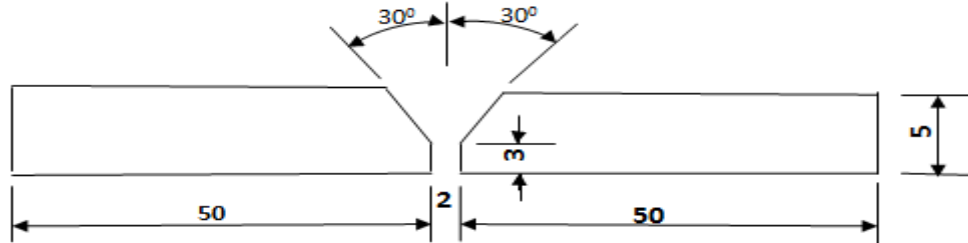
Figure 1: Sample preparation for butt (v-groove) welding
