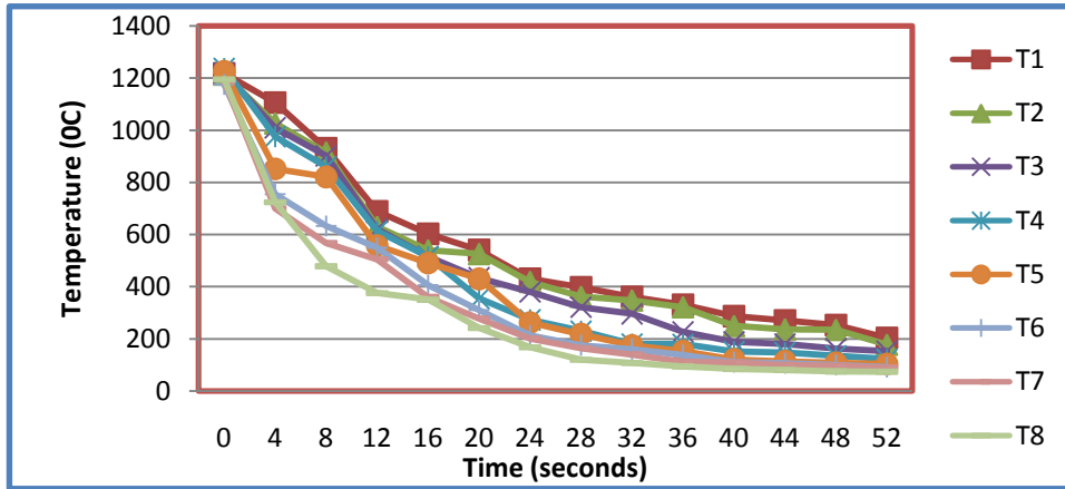
Figure 6: Impact test Curves for Water Cooled Samples
