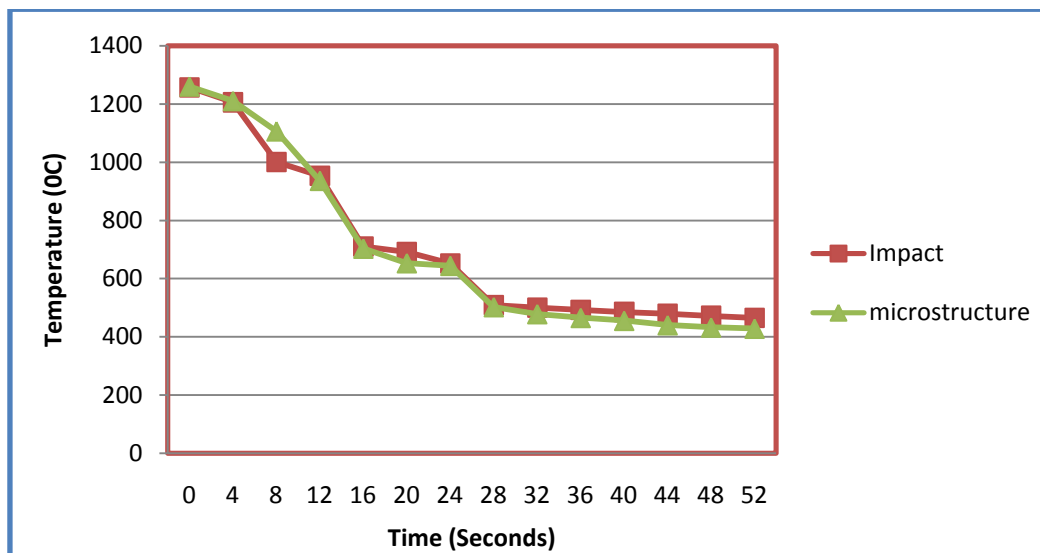
Figure 5: Air cooling curves for impact and microstructure test samples
