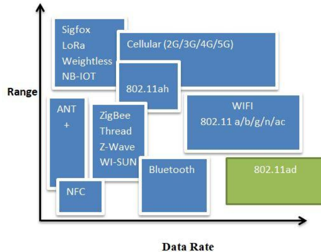
Figure No.3 IOT protocols in term of range and data rate
